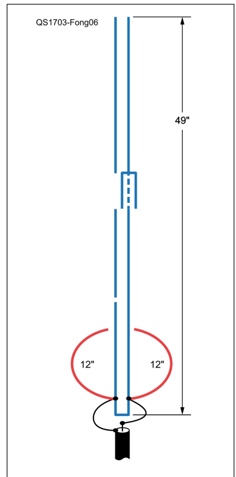
Figure 6 — The DBJ-1 dual-band J-pole with a 1.25-meter band loop antenna fed in parallel.
